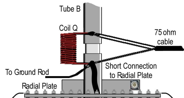
Optional Radial Plate shown installed.
